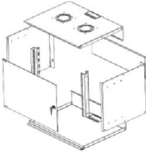
Explode View
